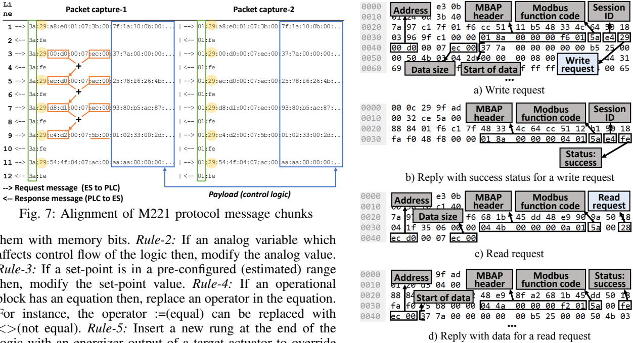
Fig. 8: Read/write message format of the M221 protocol
