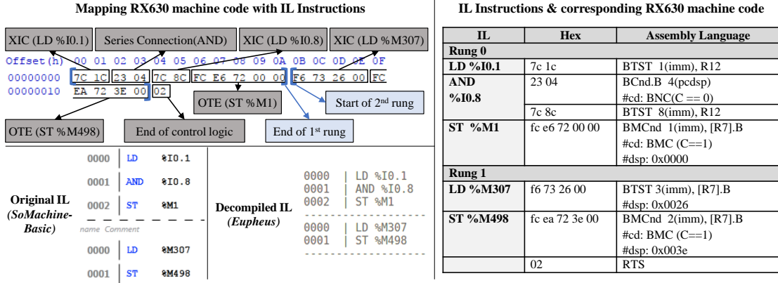
Fig. 6: Mapping RX630 machine code with IL Instructions
