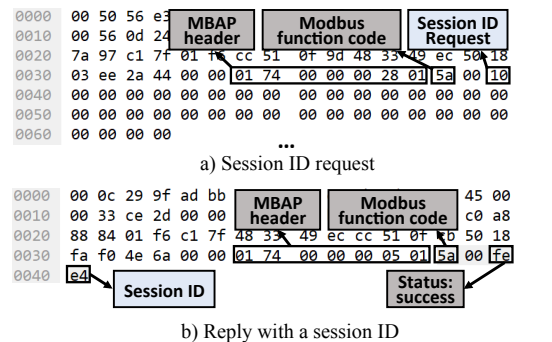
Fig. 9: Session ID request/response message format of the M221 proprietary protocol
